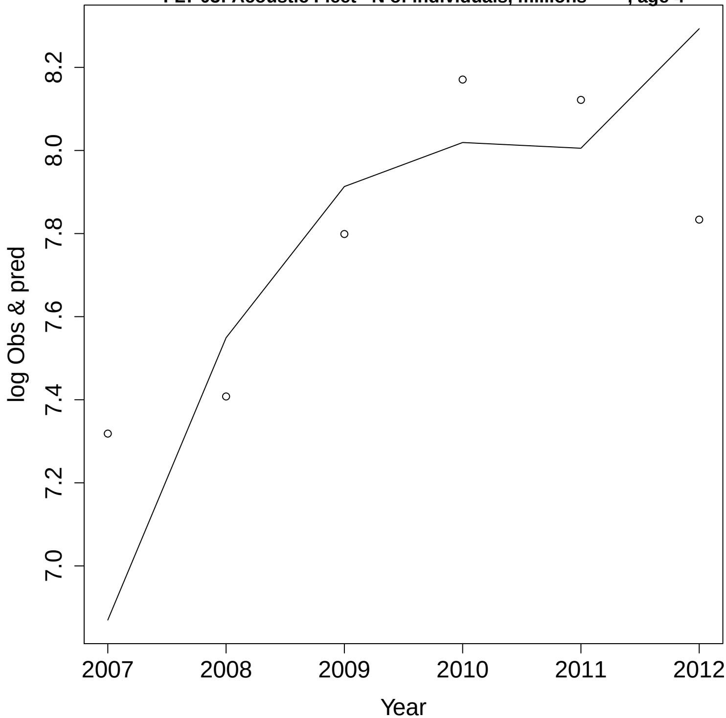
FLT 03: Acoustic Fleet N of individuals, millions, age 4
