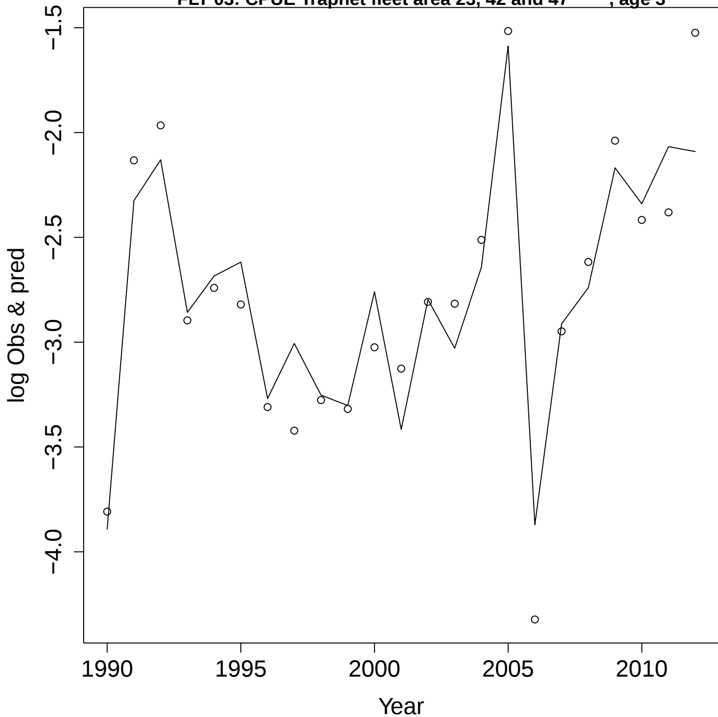
FLT 03: CPUE Trapnet fleet area 23, 42 and 47 , age 3
